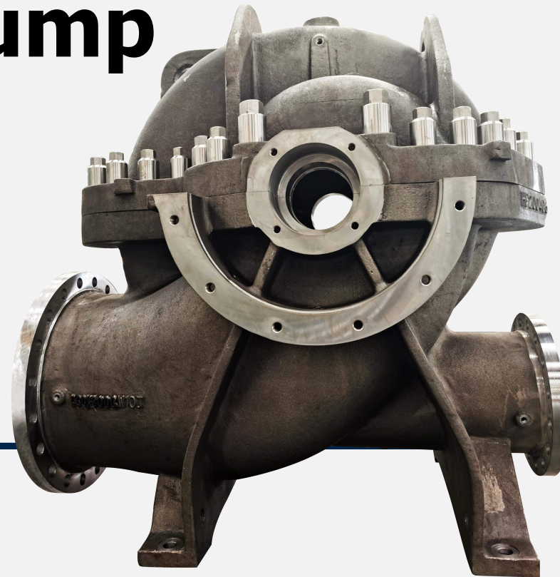
Pump Housing
